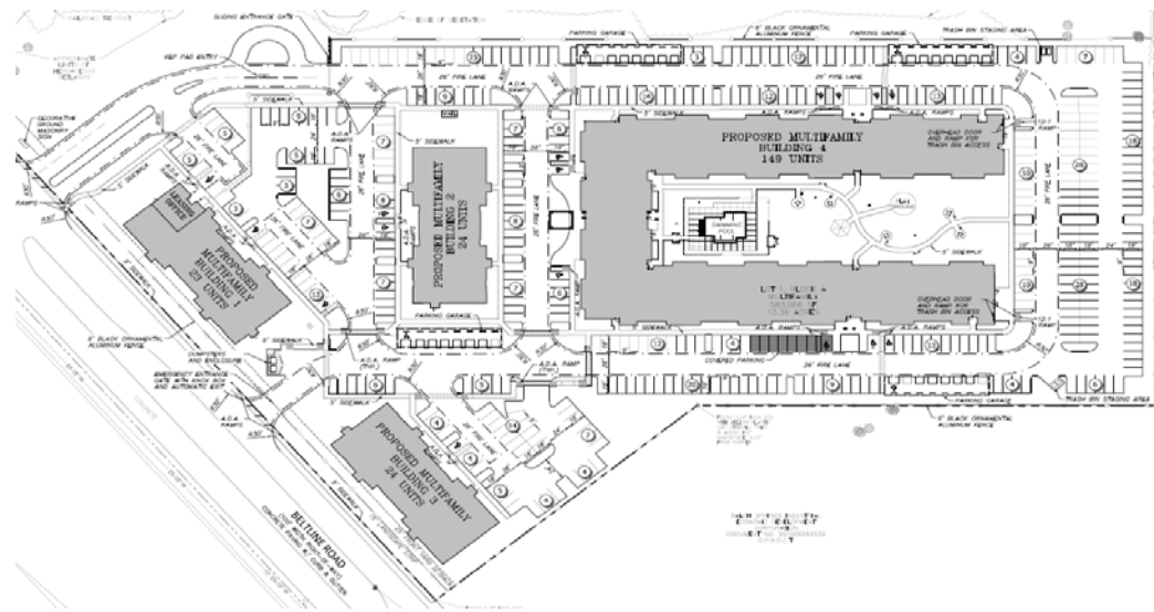
SITE PLAN
